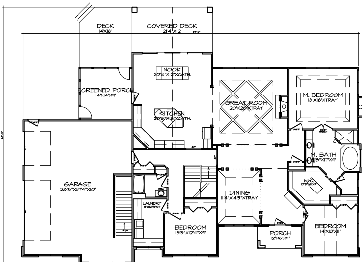
FIRST FLOOR PLAN A-4
